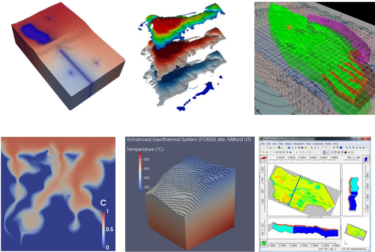
Figure (top) figures from USGS website; left: MODFLOW 6 grid example , middle: model layer visualization , right: Phreeqc-based reactive transport simulation example (bottom) left: seawater intrusion using adaptive meshing , middle: enhanced geothermal system modeling , right: USGS GUI Program ModelMuse
